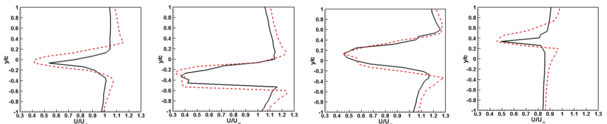
الف) \omega t = 0, 360^\circ, h = 6 \text{ cm} ب) \omega t = 90^\circ, h = 0 \text{ cm} ج) \omega t = 180^\circ, h = -6 \text{ cm} د) \omega t = 270^\circ, h = 0 \text{ cm}
